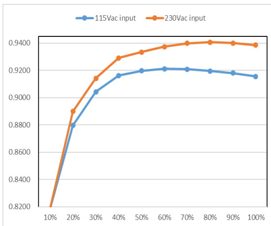
Figure 1-1. Typical efficiency Curve for 42V (1200W max)
