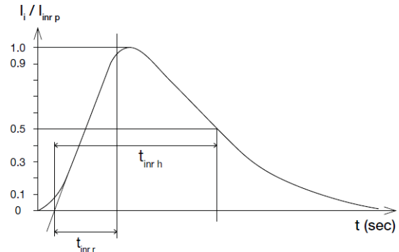
Figure 6 Inrush Current
